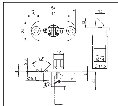
尺寸：顶部斜舌锁 GBS130/140
